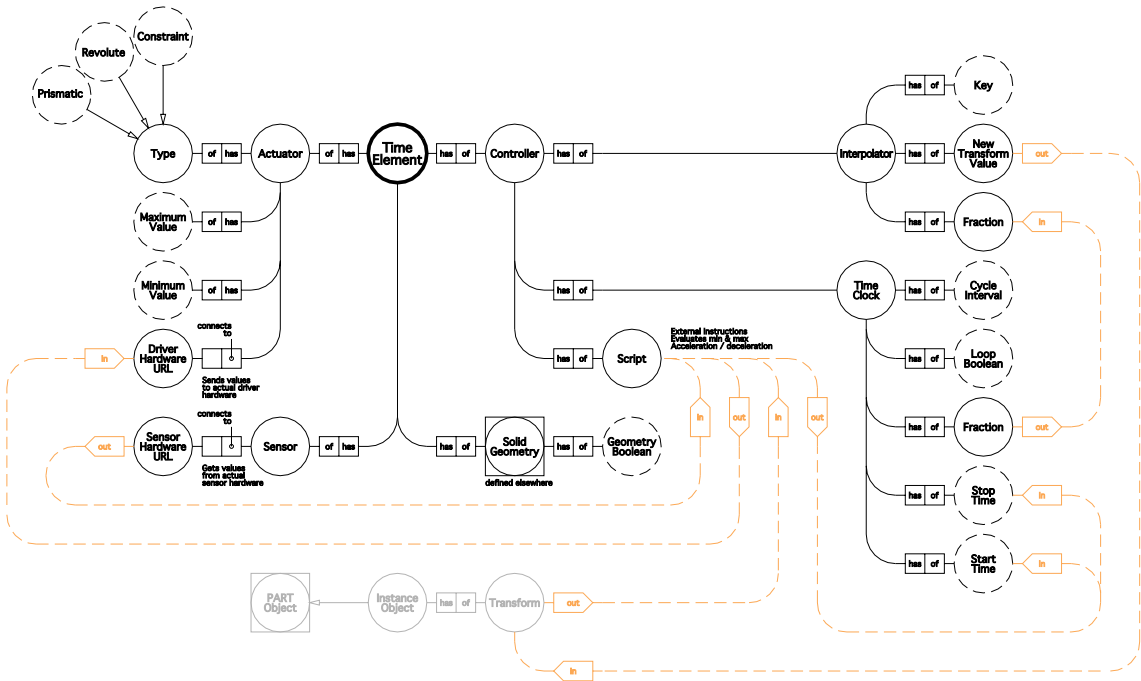
Figure 5: PARTelement extension: timeElement
